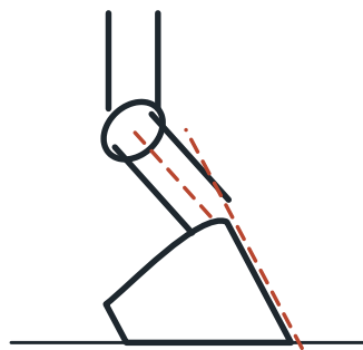
Dumped toe
